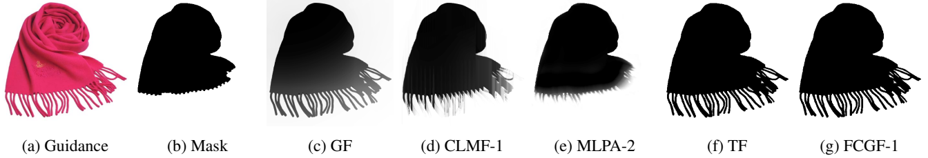
Figure 5: Image matting. A binary mask (b) is filtered under the guidance of (a). We compare FCGF-1 ( \sigma = 0.1, \epsilon = 1 ) with GF ( \sigma = 60, \epsilon = 0.1^2 ), CLMF-1 ( r = 60, \tau = 70, \epsilon = 0.1^2 ), MPLA-2 ( k = 0.005/255, \epsilon_s = 0.3, \epsilon_r = 0.1^4 ), TF ( \sigma = 0.5, \sigma_s = 10, \sigma_r = 0.05 ).
