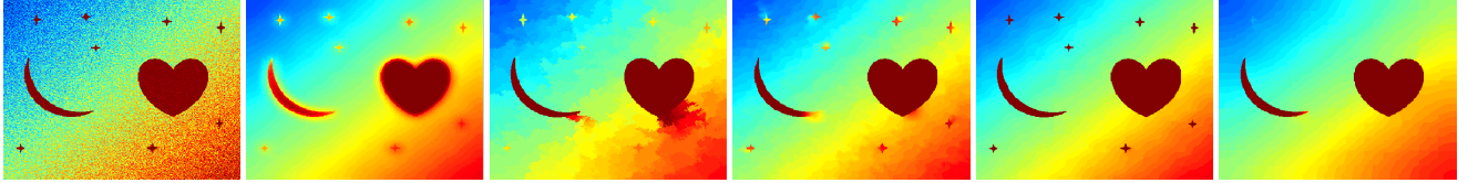
Figure 2: (a) Color visualized noisy input (PSNR=23.9dB), (b) “halo” appears around major edges (PSNR=32.1dB). (c) No “halos”, but “leaks” and “false edges” destroy the image structure (PSNR=28.4dB), (d) TF [2] just alleviates the “leak” problem, but it still appears around some object edges (35.2dB). (e) With a small smoothing window, our method could be used for denoising ( 45.5dB ), and all the object edges are preserved well. (f) Some undesirable details (“stars”) removed by using large window while other contents are preserved.
