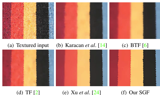
Figure 8: Texture suppression. (b)~(e) usually overly smooth some major edges in order to remove strong textures. Parameters are adjusted to prove their best performance. (f) result of our SGF ( r = 12, \sigma = 0.15, \tau = 30 , 3 iterations iterative filtering).
