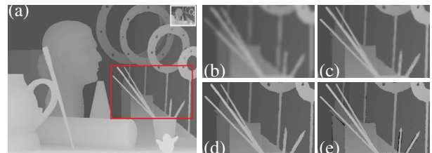
Figure 10: Depth map upsampling results. (a) low-resolution input (upper right) and 8\times upsampling result of our SGF. (b)~(e) close-up of the red window. (b) GF [13], (c) state-of-the-art, David et al. [8], (d) our SGF ( \sigma=0.05, r=16, \tau=20/255 ), (e) ground truth.
